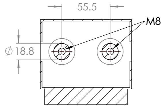
SECTION B-B SCALE 2:5
